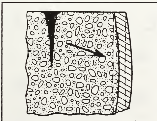
Figure 2.5 Shifting Form Crack (Reference 3)
